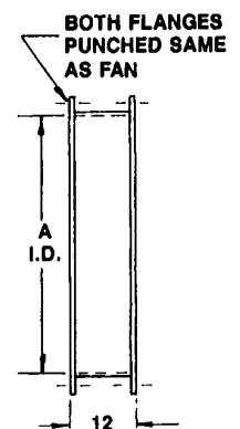
Casing Extension
